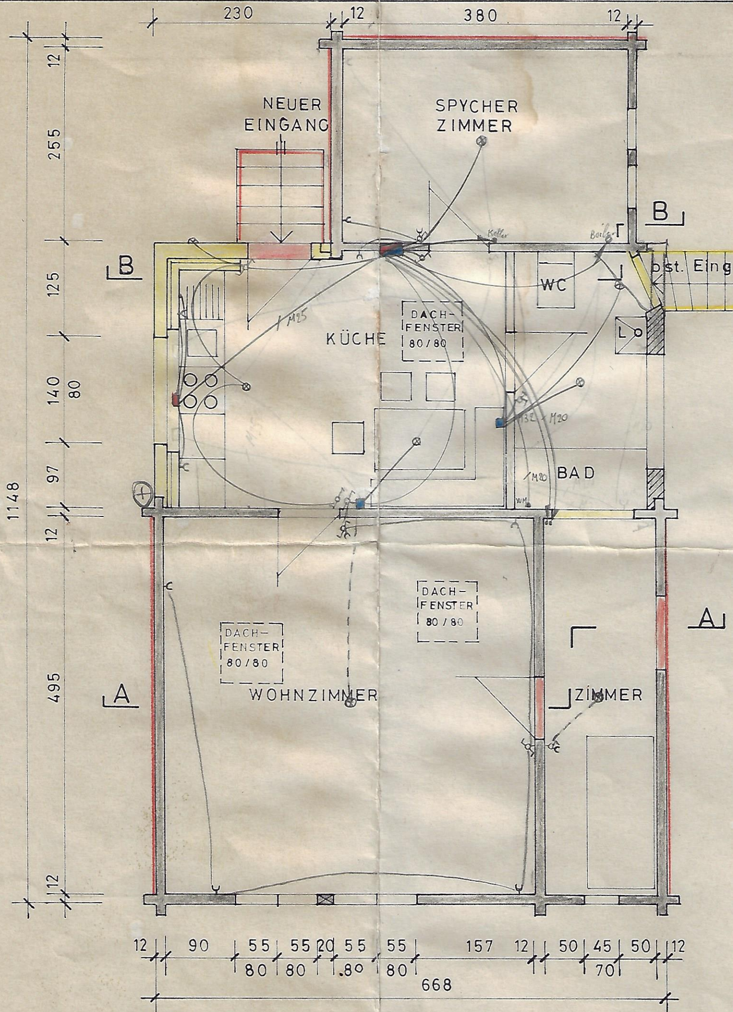
GRUNDRISS 1. STOCK
